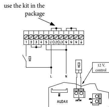
Supplementary Resistance configura- tion 6kW supplied with 230 Vac 50 Hz
