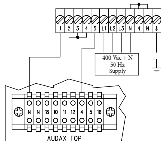
Supplementary Resistance configuration 6kW supplied with 400 Vac + N 50 Hz
