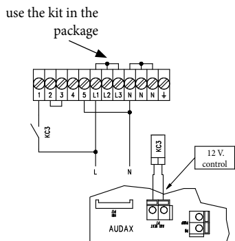
Supplementary Resistance configuration 2kW supplied with 230 Vac 50 Hz
