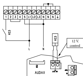
Supplementary Resistance configuration 4kW supplied with 400 Vac + N 50 Hz
