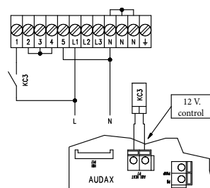
Supplementary Resistance configuration 6kW supplied with 400 Vac + N 50 Hz
