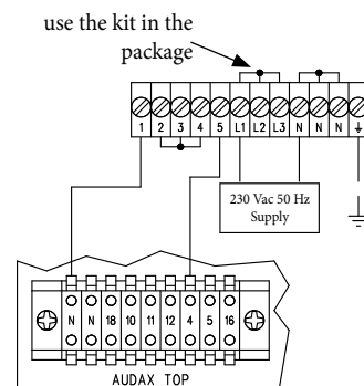
Supplementary Resistance configuration 6kW supplied with 230 Vac 50 Hz
