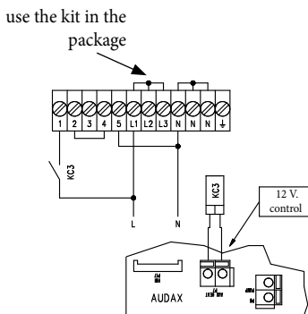
Supplementary Resistance configuration 4kW supplied with 230 Vac 50 Hz
