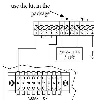
Supplementary Resistance configuration 4kW supplied with 230 Vac 50 Hz
