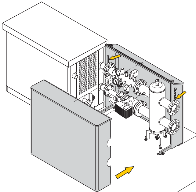
External covering kit for INAIL safety kit and complete hydraulic separator for 150-350 kW
