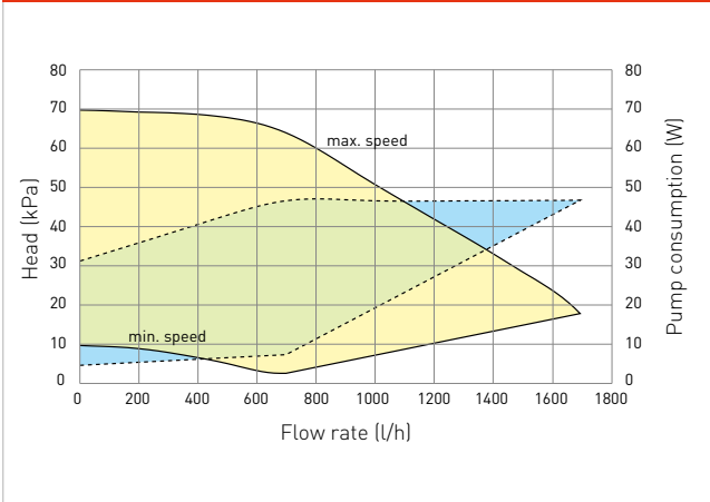
Constant head ( \Delta P C )
