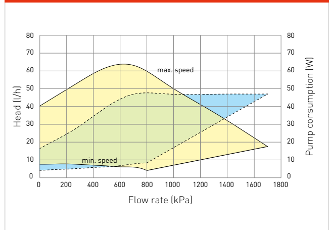
Proportional head ( \Delta P V ) with mixing valve closed
