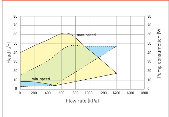
Proportional head ( \Delta P V )
