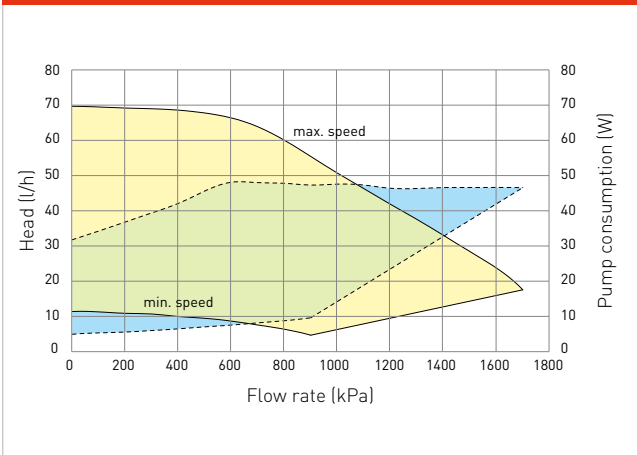
Constant head ( \Delta P C ) with mixing valve closed
