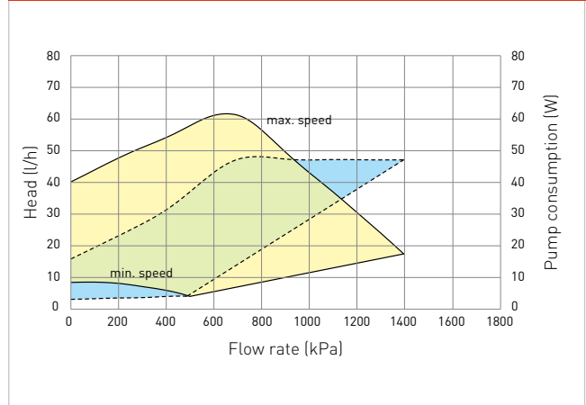
Proportional head ( \Delta P V ) with mixing valve open
