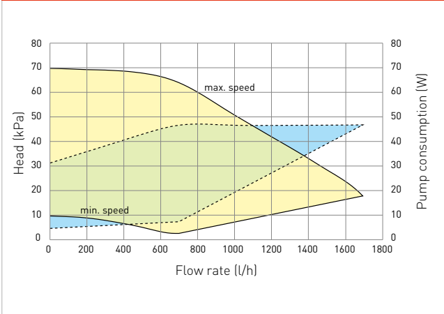
Constant head ( \Delta P C ) with mixing valve open
